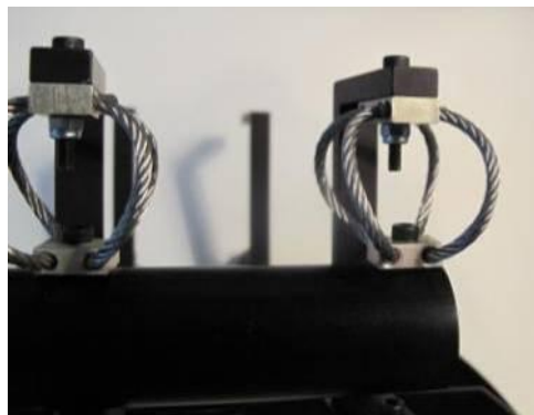
Standard mounting - No Sway Bar
