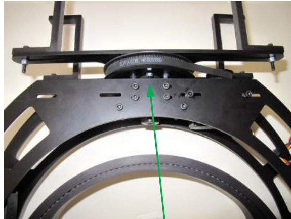
Set Screws
